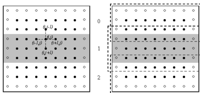
Figure 2: Data distribution
