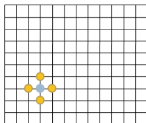
Figure 1: Jacobi method
